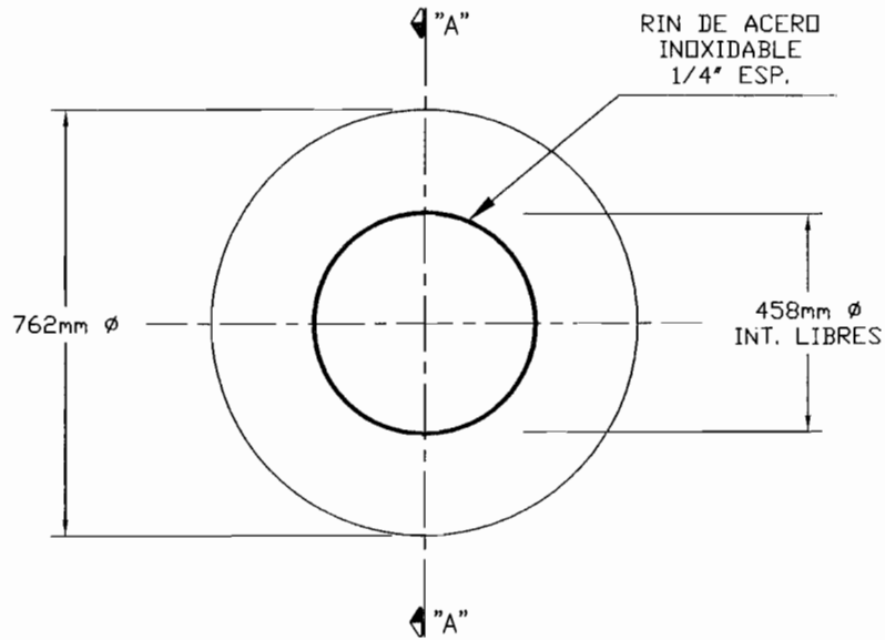
VISTA FRONTAL
